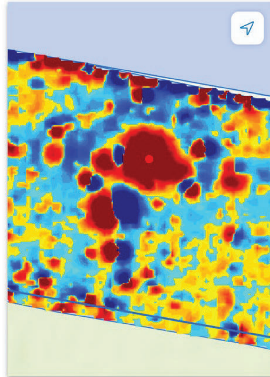
Significant object
